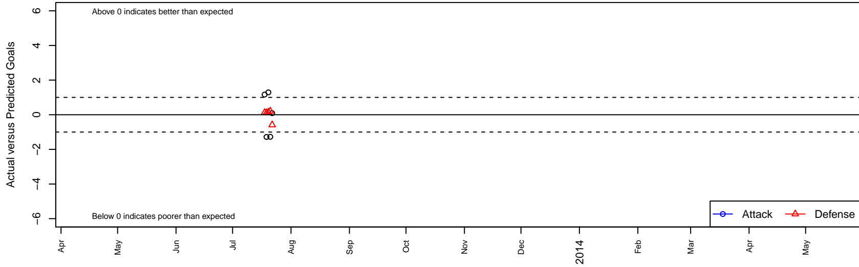
New Jersey PDA B97 Dots are actual minus expected GF (blue circles) and GA (red triangles). Blue line is smoothed change in attack strength. Red is smoothed change in defense strength.
